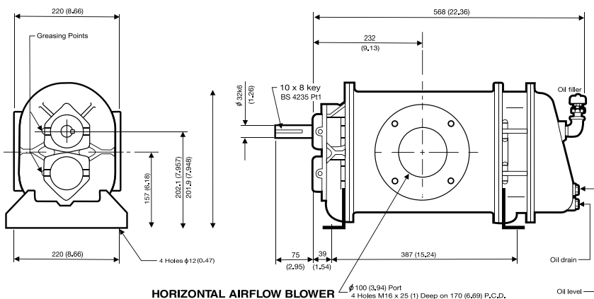
HORIZONTAL AIRFLOW BLOWER 4 Holes M16 x 25 (1) Deep on 170 (6.69) P.C.D.
