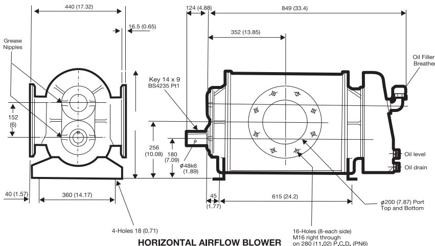
HORIZONTAL AIRFLOW BLOWER
