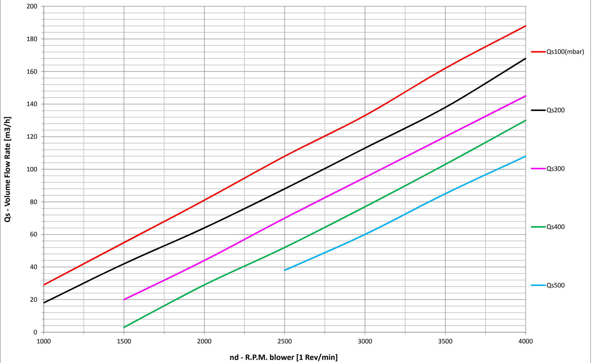
SR010-Temperature Vs R.P.M At Vacuum 100-500 mbar
