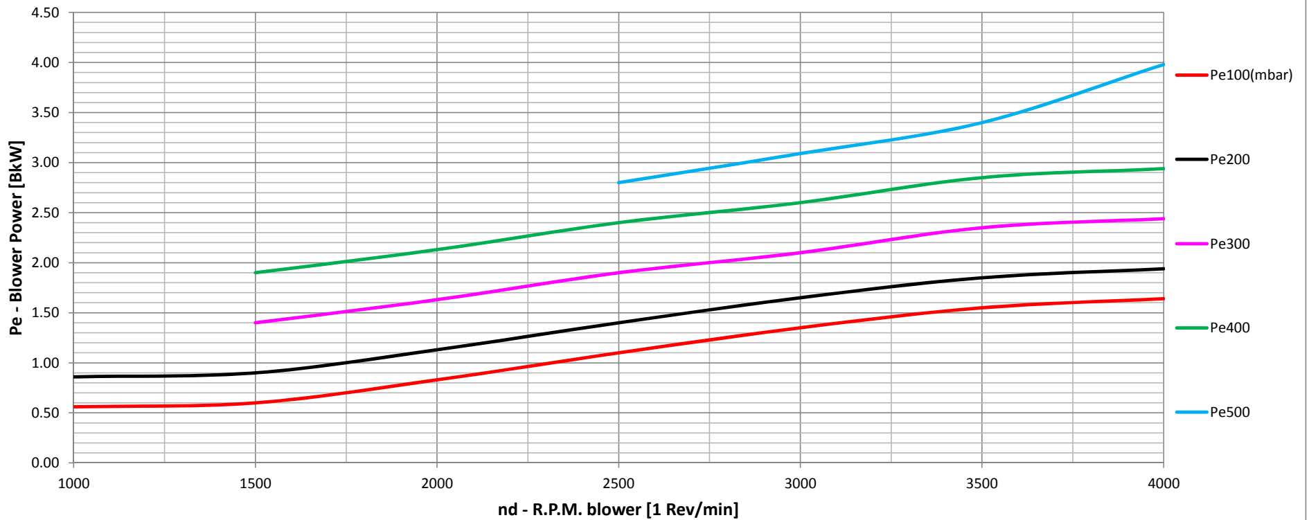
SR010-Blower Power B.K.W Vs R.P.M At Vacuum 100-500 mbar
